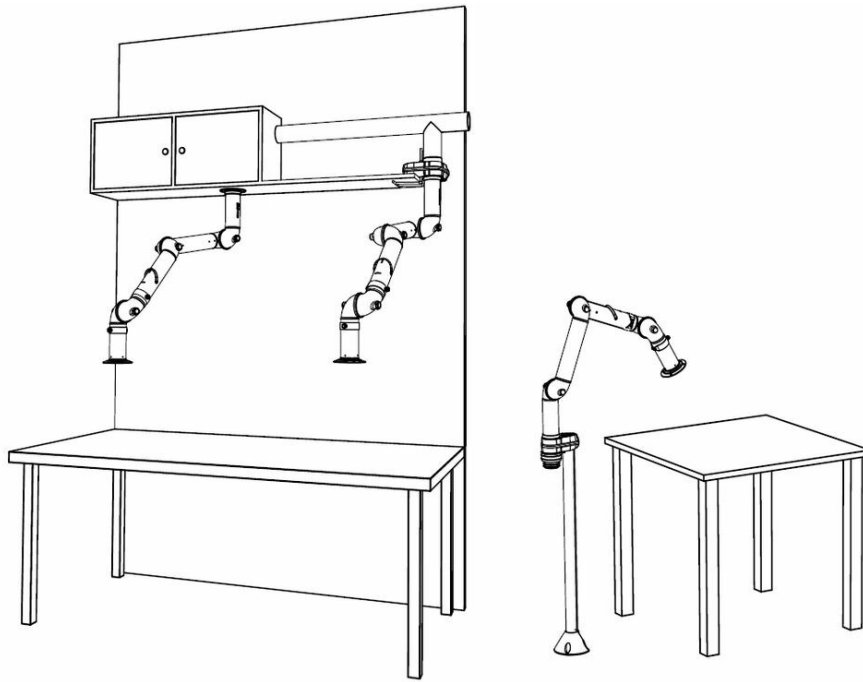
Other mounting examples: Left: Over bench cabinet mounting with FX2-Up/Down-Through arm Middle: Shelf mounting with FX2-Up-Low arm and following accessories: -FX2-Bench bracket kit Right: Floor mounting with FX2-Up-Low arm and following accessories: -FX-Classic bracket -FX-Cut2fit extension-L1100
