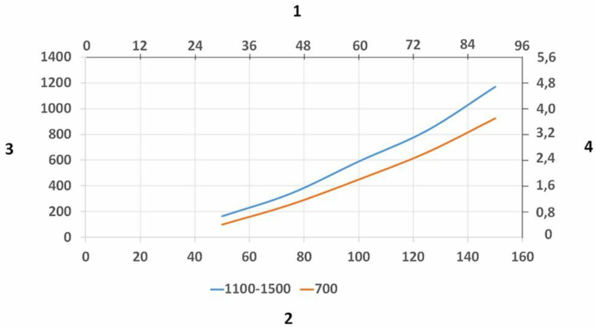
Pressure Drop diagram: 1) X- Axis: Air Flow Rate (cfm) 2) X- Axis: Air Flow Rate (m³/h) 3) Y-Axis: Static Pressure Drop (Pa) 4) Y-Axis: Static Pressure Drop (in. wg.)
