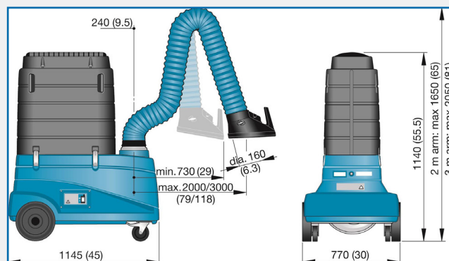
Nederman FilterCart+
