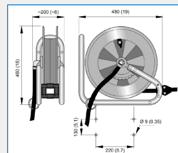
HOSE REEL 893 DIMENSIONS
