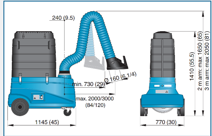
Nederman FilterCart
